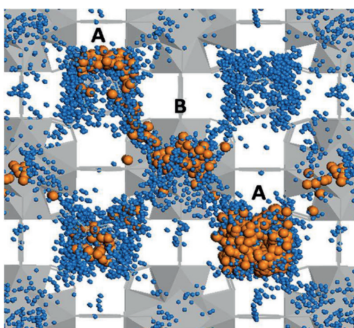
Figure 5. Illustration of the water (blue) -mediated pathway followed by the proton (orange) along the tetrahedral (A) and octahedral cages (B) of \text{UiO-66}(\text{Zr})-(\text{CO}_2\text{H})_2 . aMS-EVB3-MD simulations performed at 450 K.
